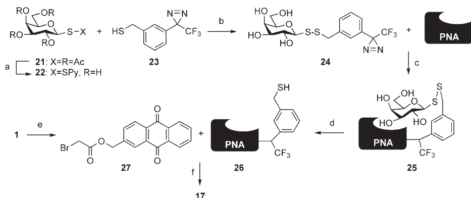
Scheme 3. Synthesis of anthraquinone–lectin hybrid 17 . Reagents and conditions: a) PySSPy, LiOH, MeOH, 54%; b) AcOH, MeOH, H_2O , 84%; c) h\nu , phosphate buffer (10 mM, pH 7.4); d) DTT, phosphate buffer (10 mM, pH 8.1, 10 mM EDTA); e) BrCH 2 COCl, 2,6-lutidine, CH 2 Cl 2 , 90%; f) DMF, phosphate buffer, (10 mM, pH 7.4). Py = pyridyl; DTT = 1,4-dithiothreitol.
