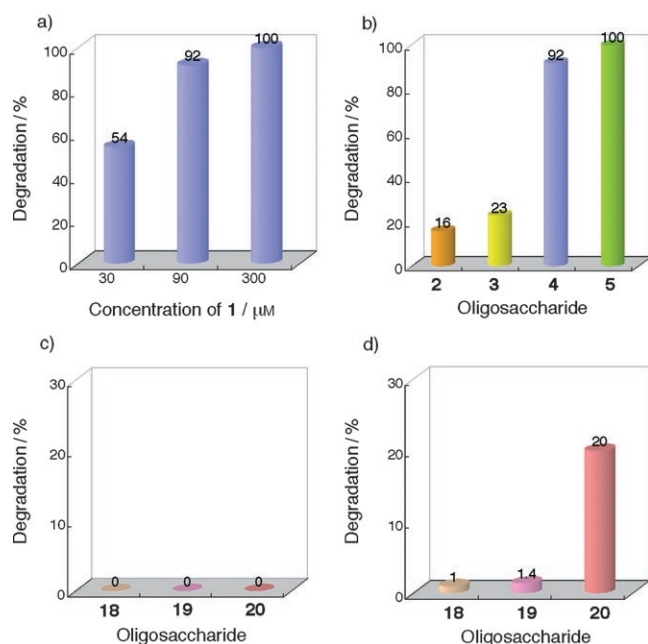
Figure 2. Photodegradation of oligosaccharides. a) \beta -CD (30 \mu M) was incubated with 1 (30, 90, and 300 \mu M) in 20% acetonitrile/ H_2O (30 \mu L) under the conditions described in Figure 1 and analyzed by HPLC (TSKgel Amide-80, 4.6 \times 250 mm; 3:2 MeCN/ H_2O ; flow rate 1.0 mL min -1 ; 30 ^{\circ} C; detection by IR). b) Maltoheptaose ( 2 ), \alpha -CD ( 3 ), \beta -CD ( 4 ), and \gamma -CD ( 5 ) at concentrations of 30 \mu M each were incubated with 1 (90 \mu M) in 20% acetonitrile/ H_2O (30 \mu L) under the conditions described in Figure 2a and analyzed by the method indicated in Figure 2a. c) Glc( \beta -1,4)Glc ( 18 ), Man( \alpha -1,3)Man ( 19 ), and Gal( \beta -1,3)GalNAc ( 20 ) at concentrations of 30 \mu M each were incubated with 1 (9 \mu M) in phosphate buffer (30 \mu L, 10 mM, pH 7.4) at 25 ^{\circ} C for 2 h under irradiation with a UV lamp (365 nm, 100 W) placed 10 cm from the mixture and analyzed by HPLC (TSKgel Amide-80, 4.6 \times 250 mm; 3:2 MeCN/ H_2O ; flow rate 0.5 mL min -1 ; 30 ^{\circ} C; detection by IR). d) Glc( \beta -1,4)Glc ( 18 ), Man( \alpha -1,3)Man ( 19 ), and Gal( \beta -1,3)GalNAc ( 20 ) at concentrations of 30 \mu M each were incubated with 17 (9 \mu M) under the conditions described in Figure 2c and analyzed by the method indicated in Figure 2c.
